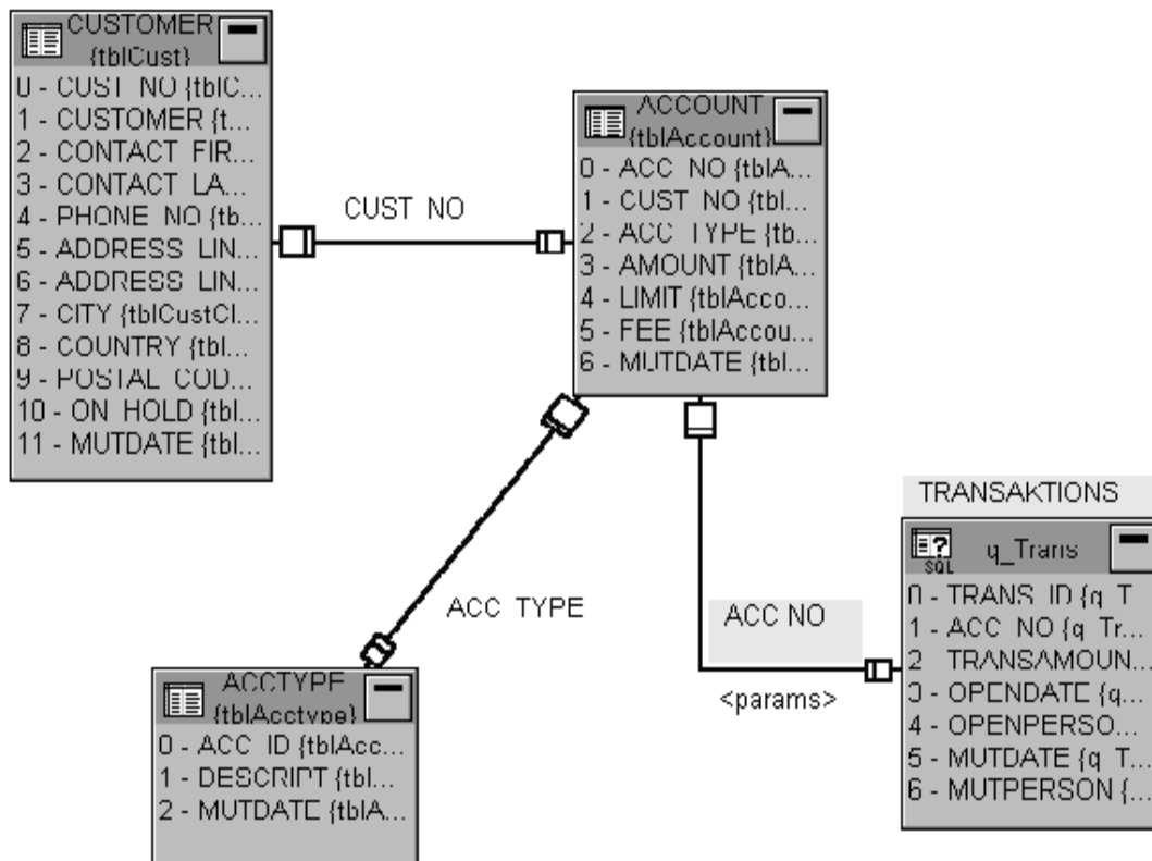
Abb. 9: ERD Diagram
