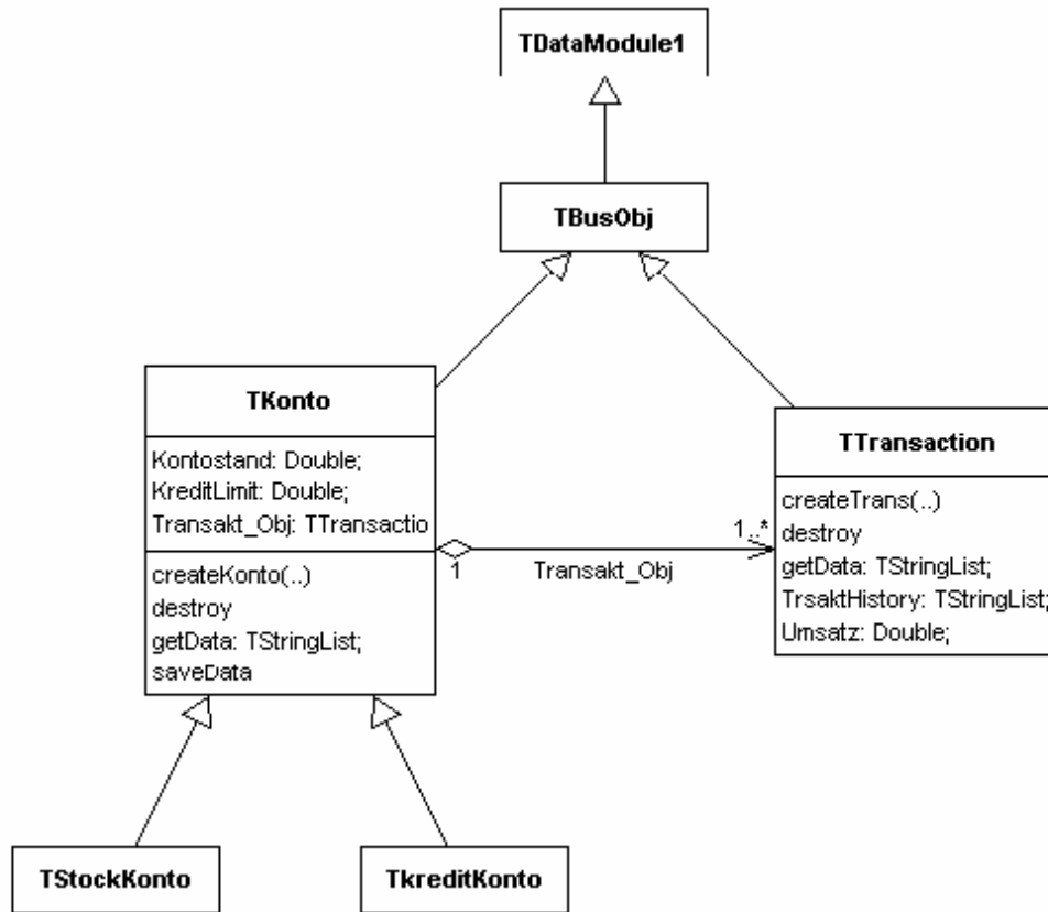
Abb. 3: Class Diagram
