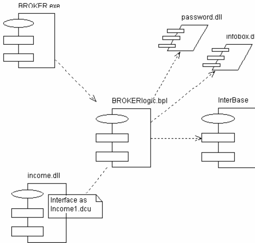
Abb. 7: Components
