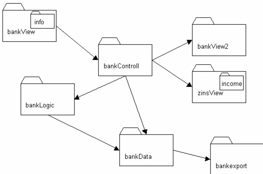
Abb. 6: Packages
