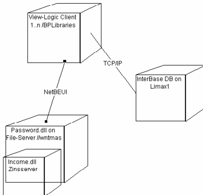
Abb. 8: Deployment
