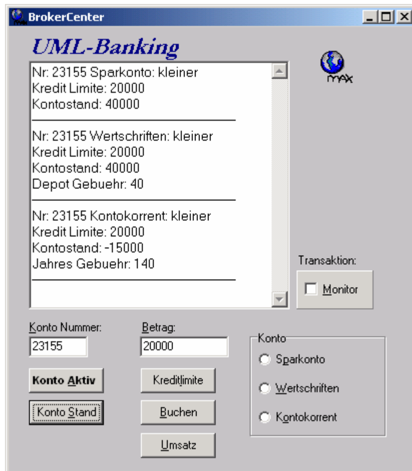
Abb. 10: GUI Design
