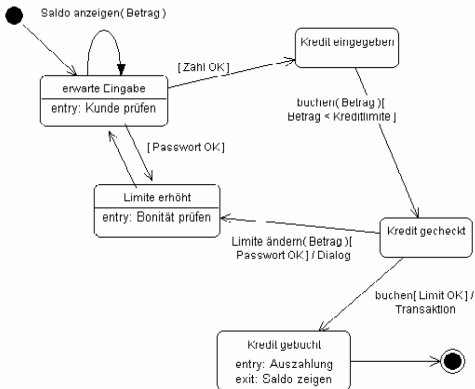
Abb. 4: State Event
