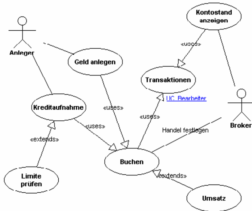
Abb.1: Use Case
