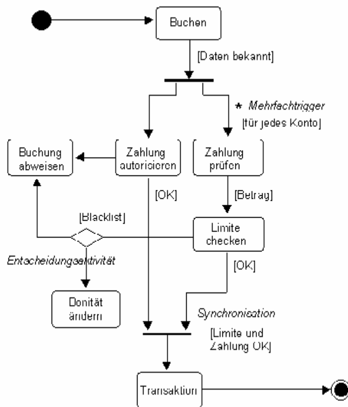
Abb. 2: Activity
